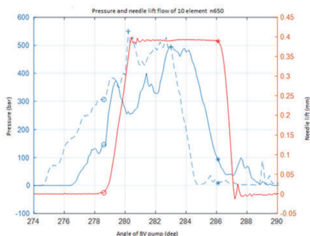
Figure 7: Pressure and needle lift flow diagram of element 10 at a BV pump speed of 650 \text{min}^{-1}
