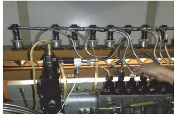
Figure 3: High pressure pipes with original engine and a special assembly (indicated by an arrow) for measuring the stroke of the injector needle
