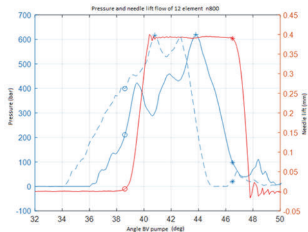
Figure 14: Pressure and needle lift flow diagram of element 12 at a BV pump speed of 800 \text{ min}^{-1}
