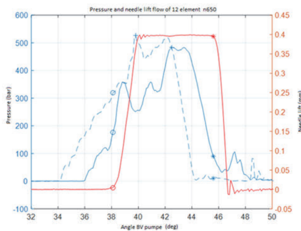
Figure 13: Pressure and needle lift flow diagram of element 12 at a BV pump speed of 650 \text{ min}^{-1}
