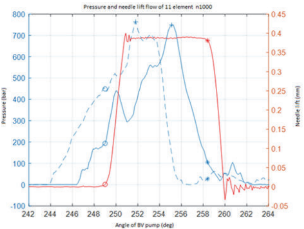
Figure 12: Pressure and needle lift flow diagram of element 11 at a BV pump speed of 1000 \text{ min}^{-1}
