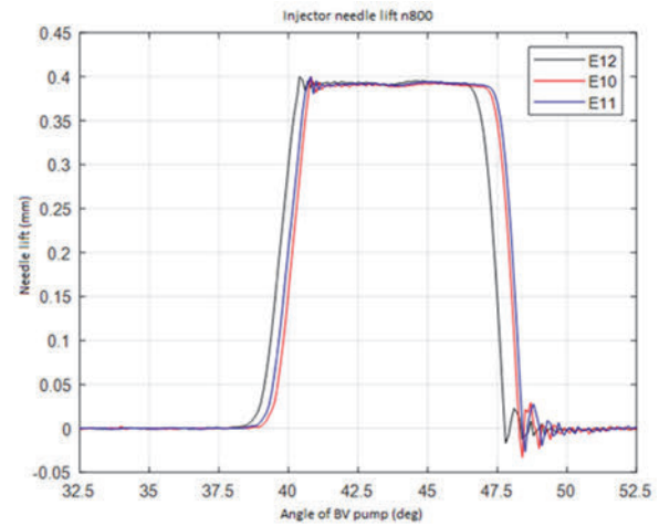
Figure 21: Injector needle lift diagrams at a BV pump speed of 800 \text{ min}^{-1}
