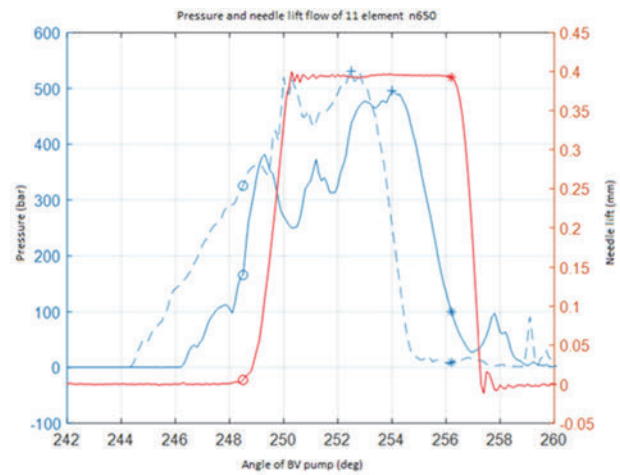
Figure 10: Pressure and needle lift flow diagram of element 11 at a BV pump speed of 650 \text{ min}^{-1}
