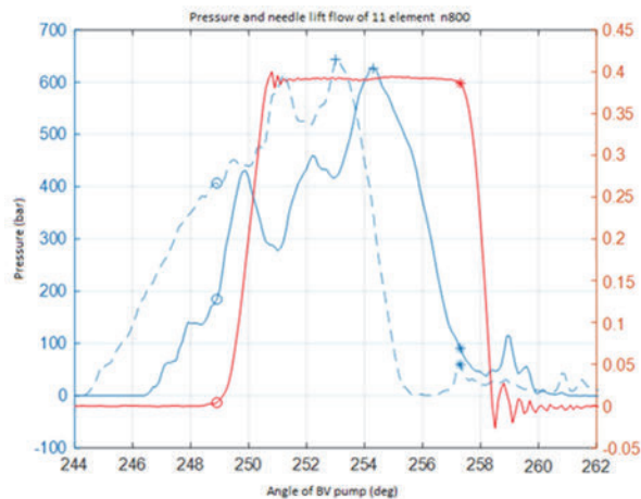
Figure 11: Pressure and needle lift flow diagram of element 11 at a BV pump speed of 800 \text{ min}^{-1}
