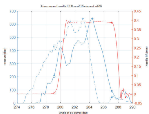
Figure 8: Pressure and needle lift flow diagram of element 10 at a BV pump speed of 800 \text{min}^{-1}
