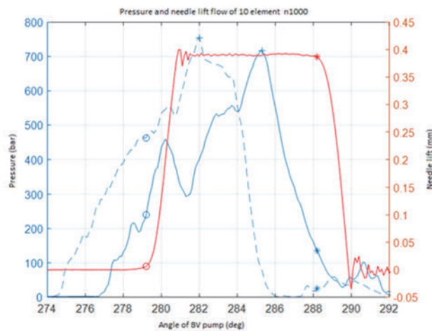
Figure 9: Pressure and needle lift flow diagram of element 10 at a BV pump speed of 1000 \text{ min}^{-1}
