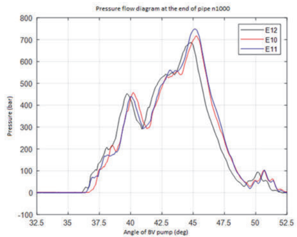
Figure 23: Pressure flow diagram at the end of pipe at a BV pump speed of 1000 \text{ min}^{-1}
