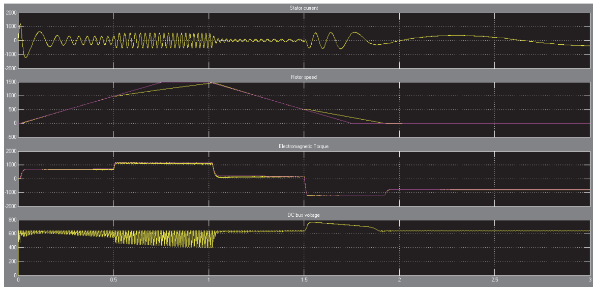
Figure 14: Changes in the stator current, rotation speed and electromagnetic moment of the electric motor and DC bus voltage of the direct current medium of the inverter EMU for \omega_r = 1500 rpm and T_m = \pm 792 Nm.
