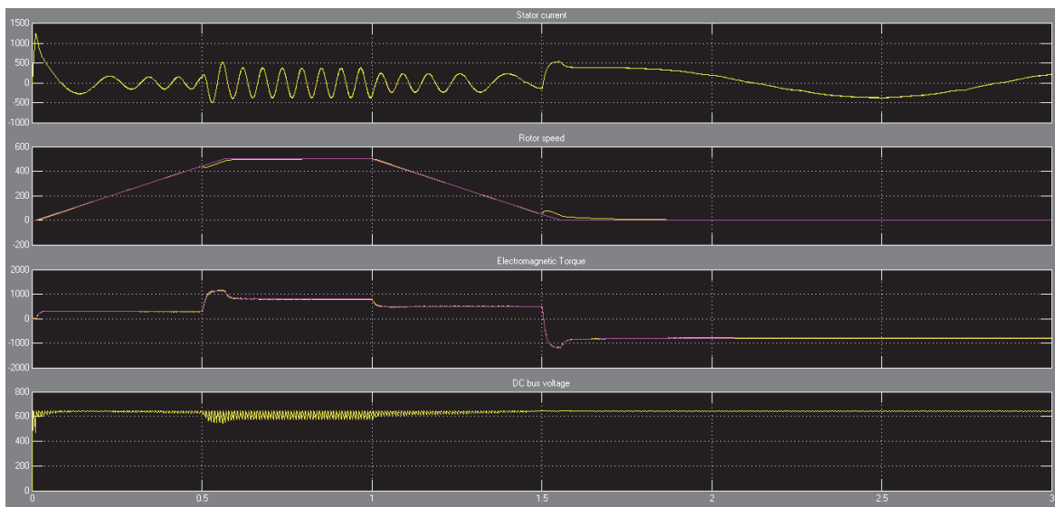
Figure 15: Changes in the stator current, rotation speed and electromagnetic moment of the electric motor and DC bus voltage of the direct current medium of the inverter EMU for \omega_r = 500 rpm and T_m = \pm 792 Nm.
