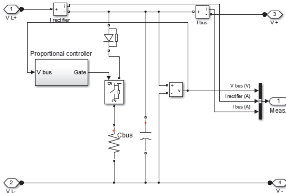
Figure 10: Simulink model of braking chopper
