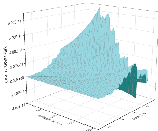
Figure 7: The transverse vibration of controlling lever
