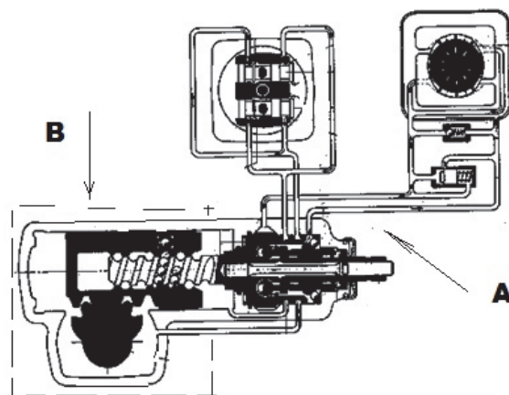
Figure 2. The scheme of the servo steering system
