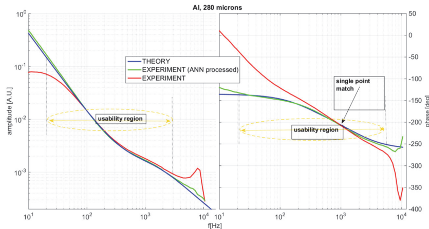
Figure 7: Theoretically obtained PA response of aluminum at 280 \mu\text{m} (blue line) vs. experimentally gained data (red line) vs. ANN-corrected experimental data (green line), [32]
