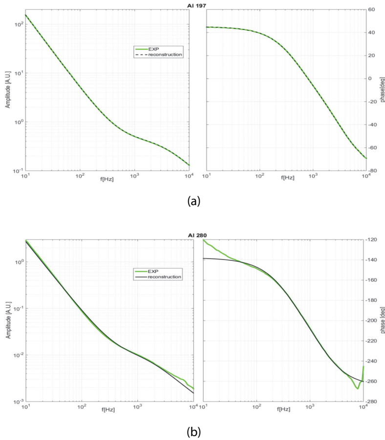
Figure 8: ANN preprocessed experimental results (green) obtained from a 197 μm (a) and 280 μm (b) thick sample alongside reconstructed data, based on the estimated parameters (black) [32]
