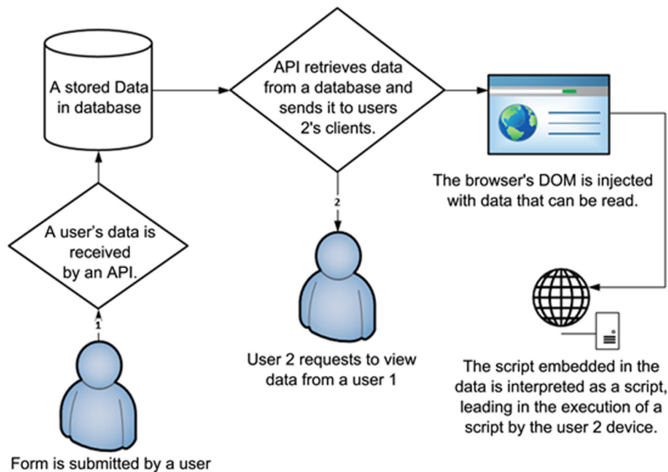
Figure 2: Stored XSS attack scenario
