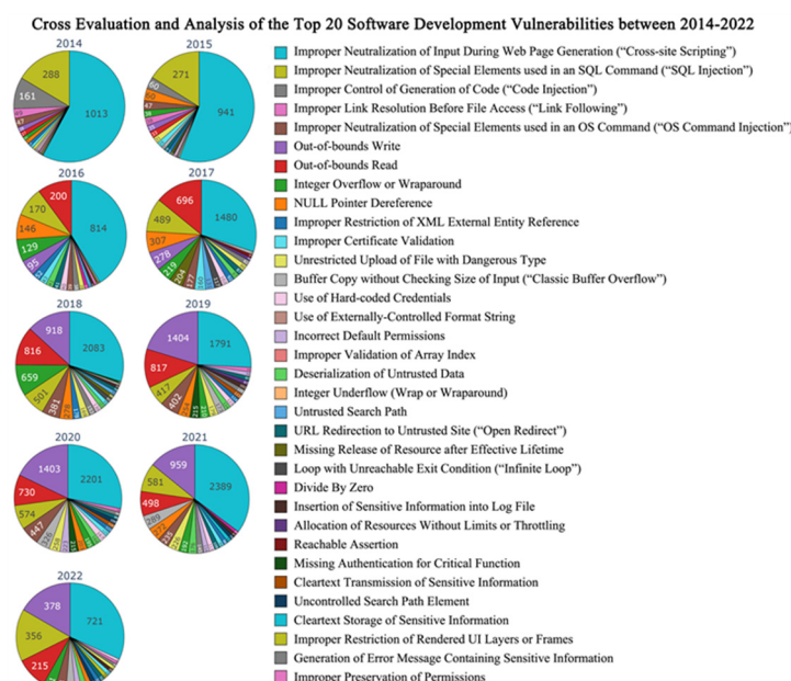
Figure 1: Comparative analysis of yearly XSS vulnerability trends (2014–2022)
